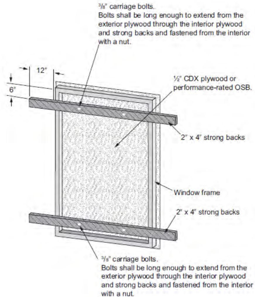
FIGURE A103.1(1) BOARDING OF DOOR OR WINDOW
