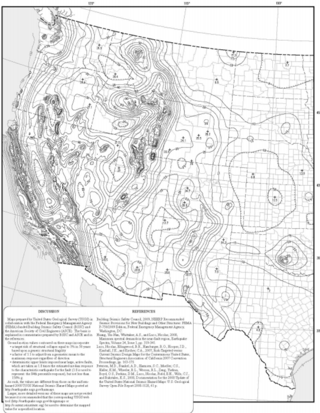
FIGURE 1613.32.1(1) RISK-TARGETED MAXIMUM CONSIDERED EARTHQUAKE (MCE R ) GROUND MOTION RESPONSE ACCELERATIONS FOR THE CONTERMINOUS UNITED STATES OF 0.2- SECOND SPECTRAL RESPONSE ACCELERATION (5% OF CRITICAL DAMPING), SITE CLASS B
