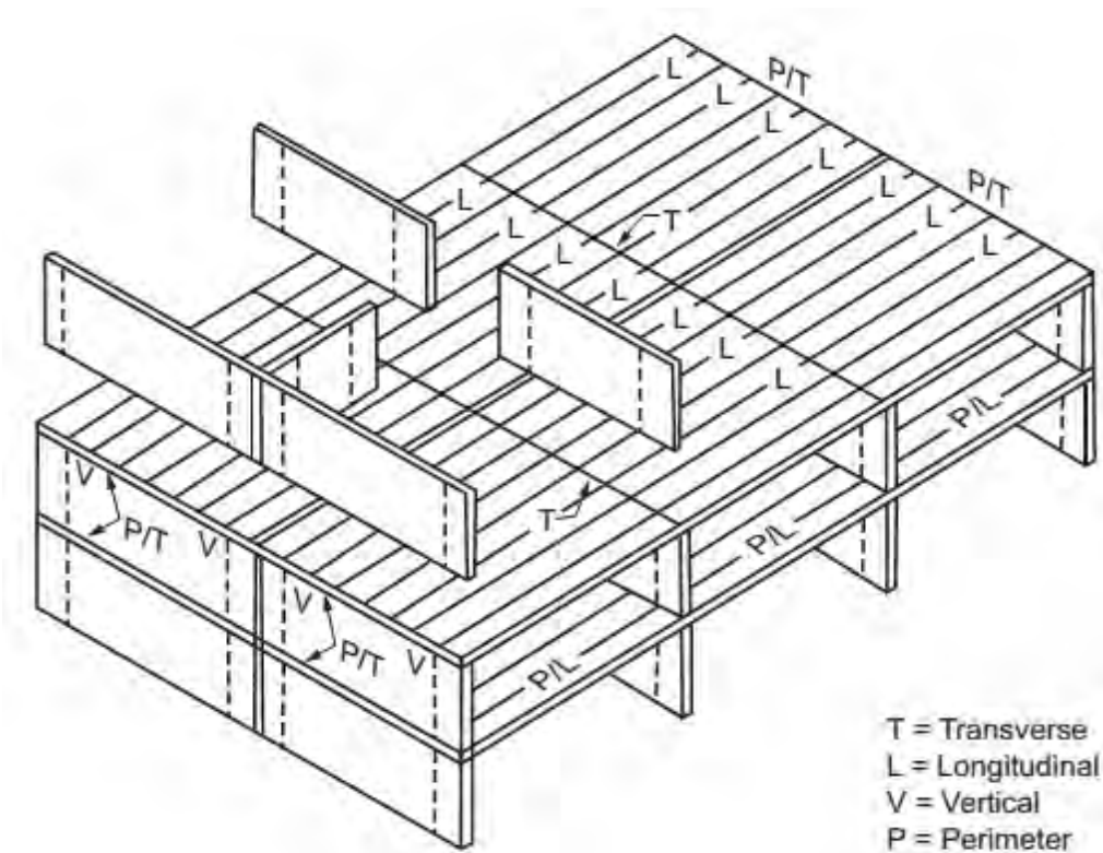
FIGURE 1615.4.3 LONGITUDINAL, PERIMETER, TRANSVERSE AND VERTICAL TIES
