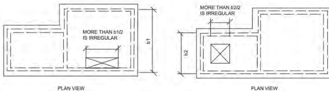
FIGURE 2308.4.4.1(2) OPENING LIMITATIONS FOR FLOOR AND ROOF DIAPHRAGMS
