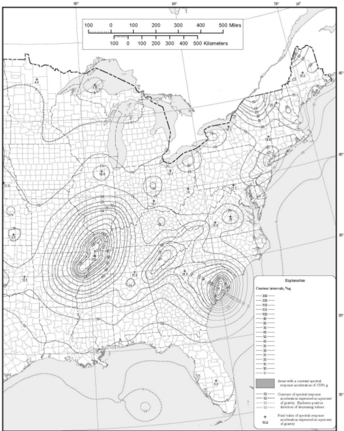
FIGURE 1613.32.1(1)-continued RISK-TARGETED MAXIMUM CONSIDERED EARTHQUAKE (MCE R ) GROUND MOTION RESPONSE ACCELERATIONS FOR THE CONTERMINOUS UNITED STATES OF 0.2- SECOND SPECTRAL RESPONSE ACCELERATION (5% OF CRITICAL DAMPING), SITE CLASS B
