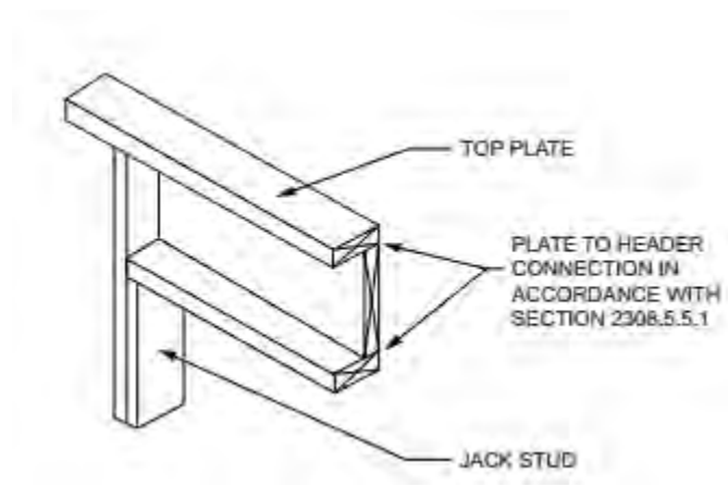
FIGURE 2308.5.5.1(2) ALTERNATIVE SINGLE-MEMBER HEADER WITHOUT CRIPPLE
