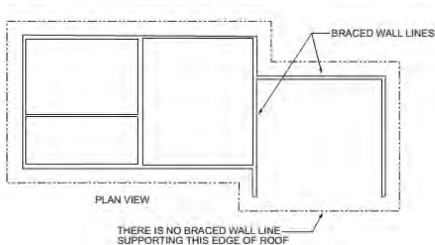
FIGURE 2308.6.8.2(1) ROOF IN SDC D OR E NOT SUPPORTED ON ALL EDGES
