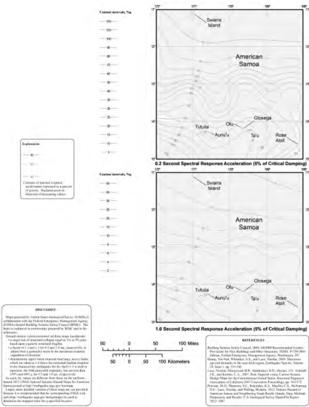
FIGURE 1613.32.1(8) RISK-TARGETED MAXIMUM CONSIDERED EARTHQUAKE (MCE R ) GROUND MOTION RESPONSE ACCELERATIONS FOR AMERICAN SAMOA OF 0.2- AND 1-SECOND SPECTRAL RESPONSE ACCELERATION (5% OF CRITICAL DAMPING), SITE CLASS B
