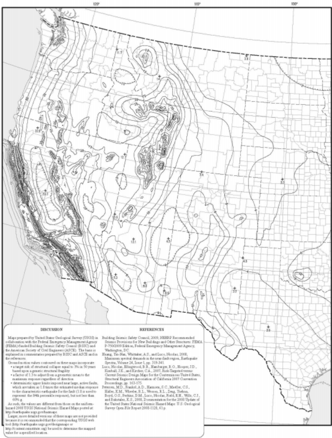
FIGURE 1613.32.1(2) RISK-TARGETED MAXIMUM CONSIDERED EARTHQUAKE (MCE R ) GROUND MOTION RESPONSE ACCELERATIONS FOR THE CONTERMINOUS UNITED STATES OF 1-SECOND SPECTRAL RESPONSE ACCELERATION (5% OF CRITICAL DAMPING), SITE CLASS B
