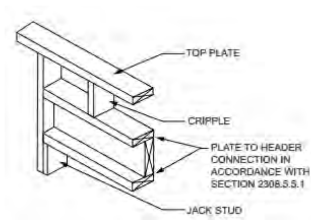
FIGURE 2308.5.5.1(1) SINGLE-MEMBER HEADER IN EXTERIOR BEARING WALL
